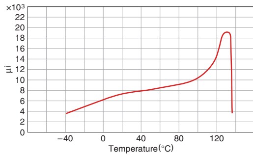
\mu_i temperature characteristics(Typ.)
