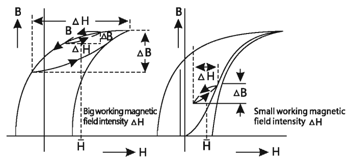
Where is the hysteresis loop, After folding between DC magnetic field and AC field with \Delta H/2
