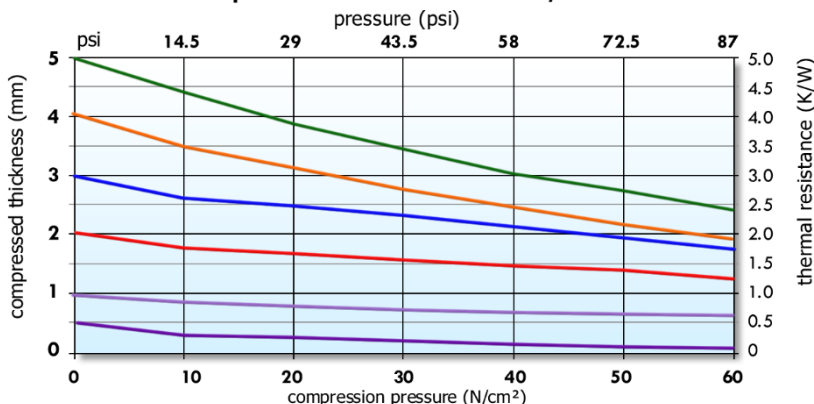
Compressibilities of Softtherm 86/225
