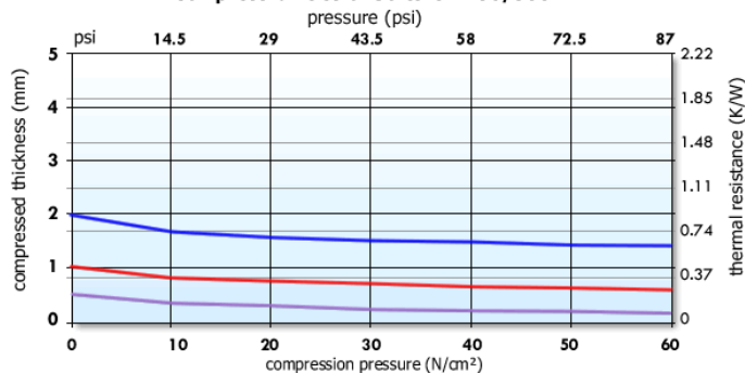
Compressibilities of Softtherm 86/500
