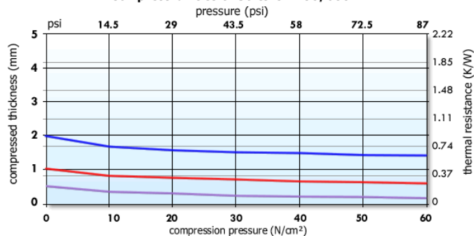
Compressibilities of Softtherm 86/600
