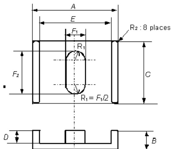
Fig.1 ELH core
