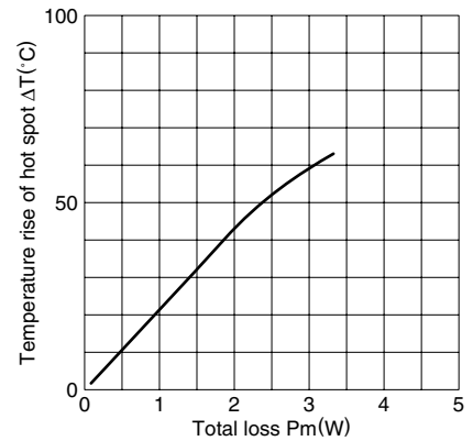
Temperature rise vs. Total loss for EI30 core (Typical) (Ambient temperature: 25°C)
