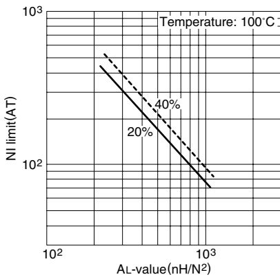
NI limit vs. AL-value for PC40ETD49 gapped core (Typical)
