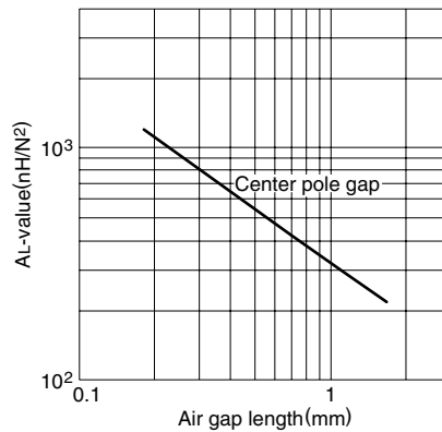
AL-value vs. Air gap length for PC40ETD49 core (Typical)
