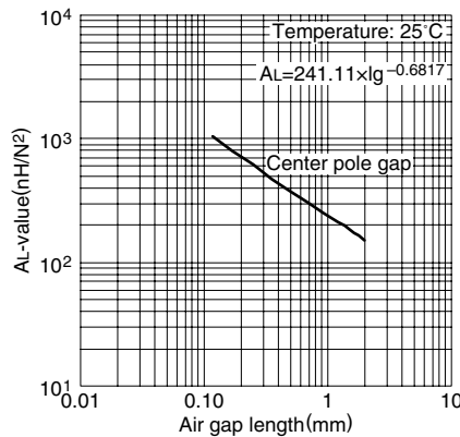
AL-value vs. Air gap length for PC40EI30 core (Typical)
