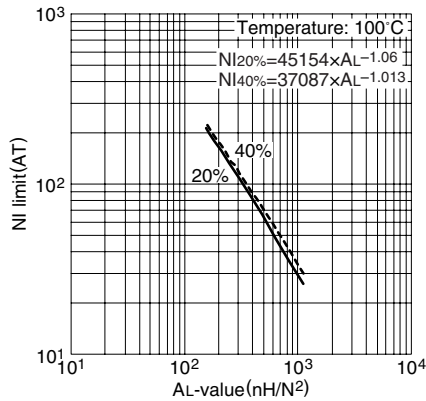
NI limit vs. AL-value for PC40EI30 gapped core (Typical)
